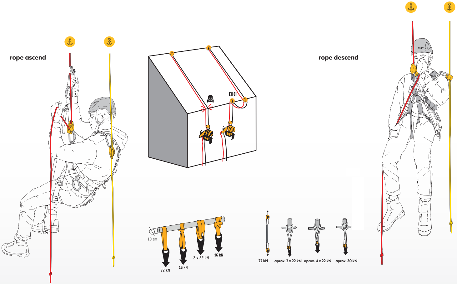
Position body into the descender and ascenders, re-place the fall arrester.
